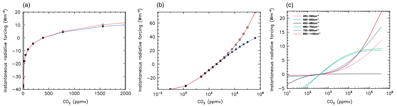
Figure 6. (a) Instantaneous Radiative Forcing of CO 2 (relative to the present-day concentration) as a function of volume mixing ratio. The red curve is for the whole infrared region, 0–3000 cm -1 . The blue curve covers only the spectral region 550–800 cm -1 (i.e. the 15 μm band). (b) As (a) but extending to higher CO 2 mixing ratios and presented against the logarithm of volume mixing ratio. (c) Radiative Forcing against CO 2 mixing ratio for the six spectral intervals.
