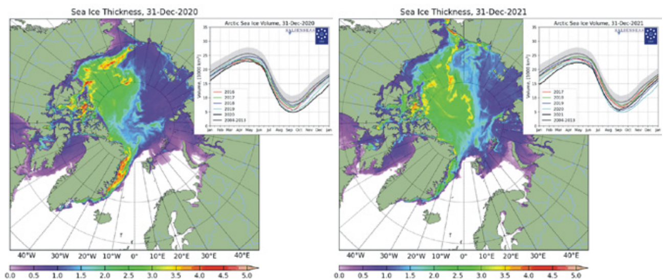
Figure 41: Arctic sea ice 2020 versus 2021
