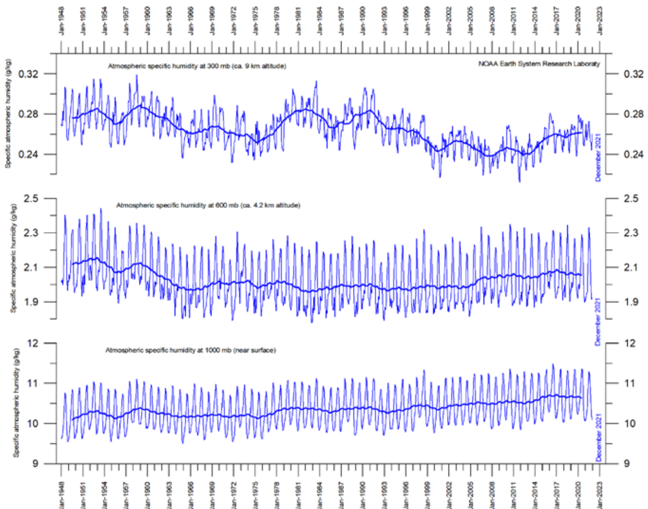
Figure 17: Humidity.
