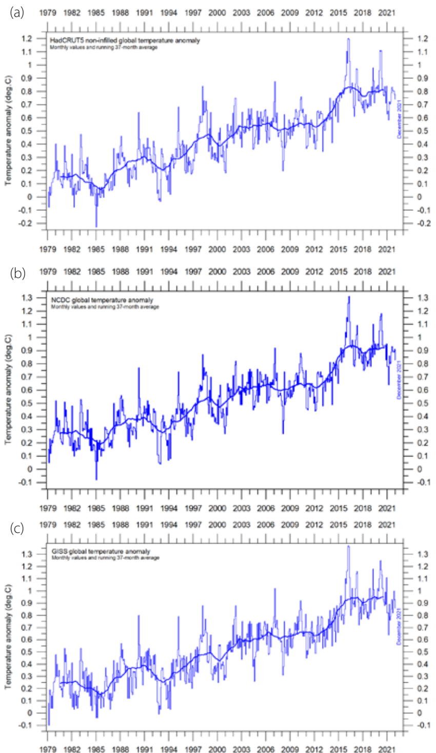
Figure 6: Global mean monthly surface air temperatures since 1979.
