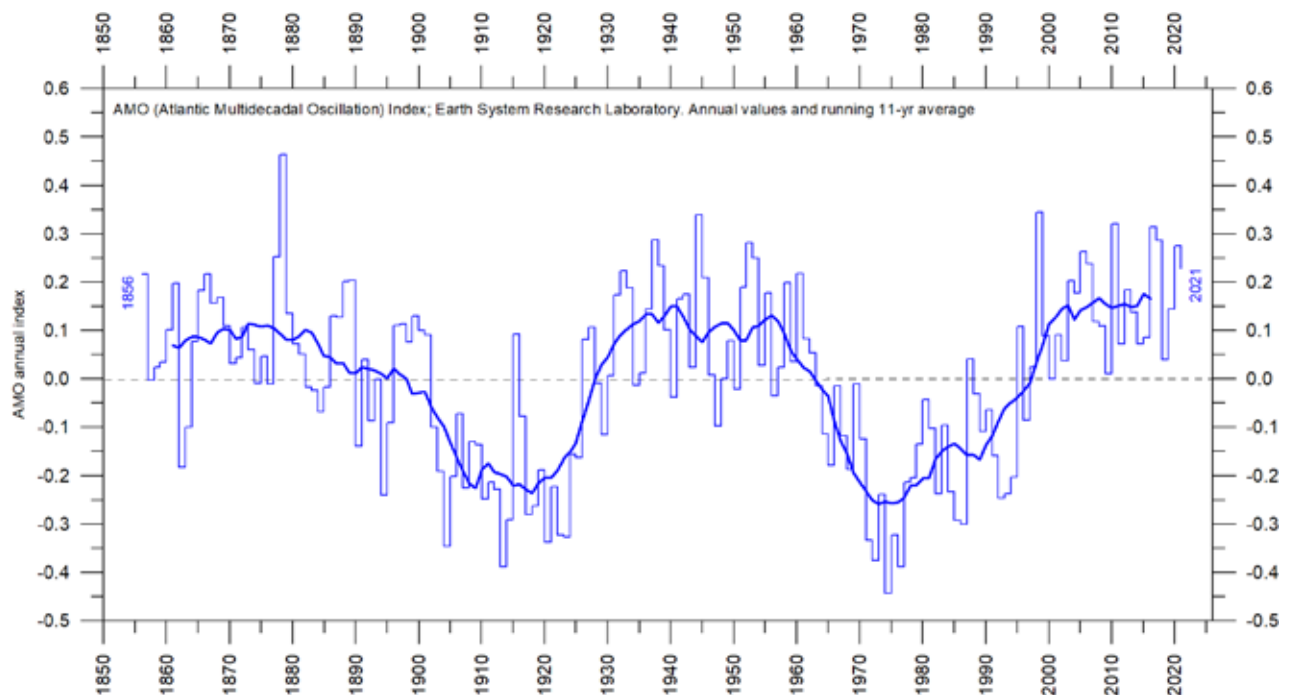
Figure 35: The Atlantic Multidecadal Oscillation
