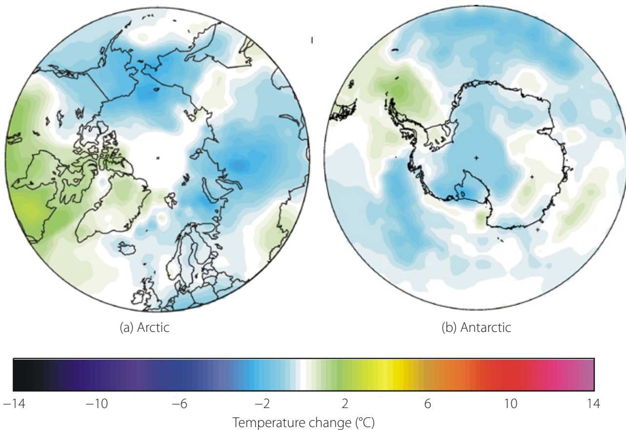
Figure 2: 2021 polar surface air temperatures compared to the average for the previous 10 years.
