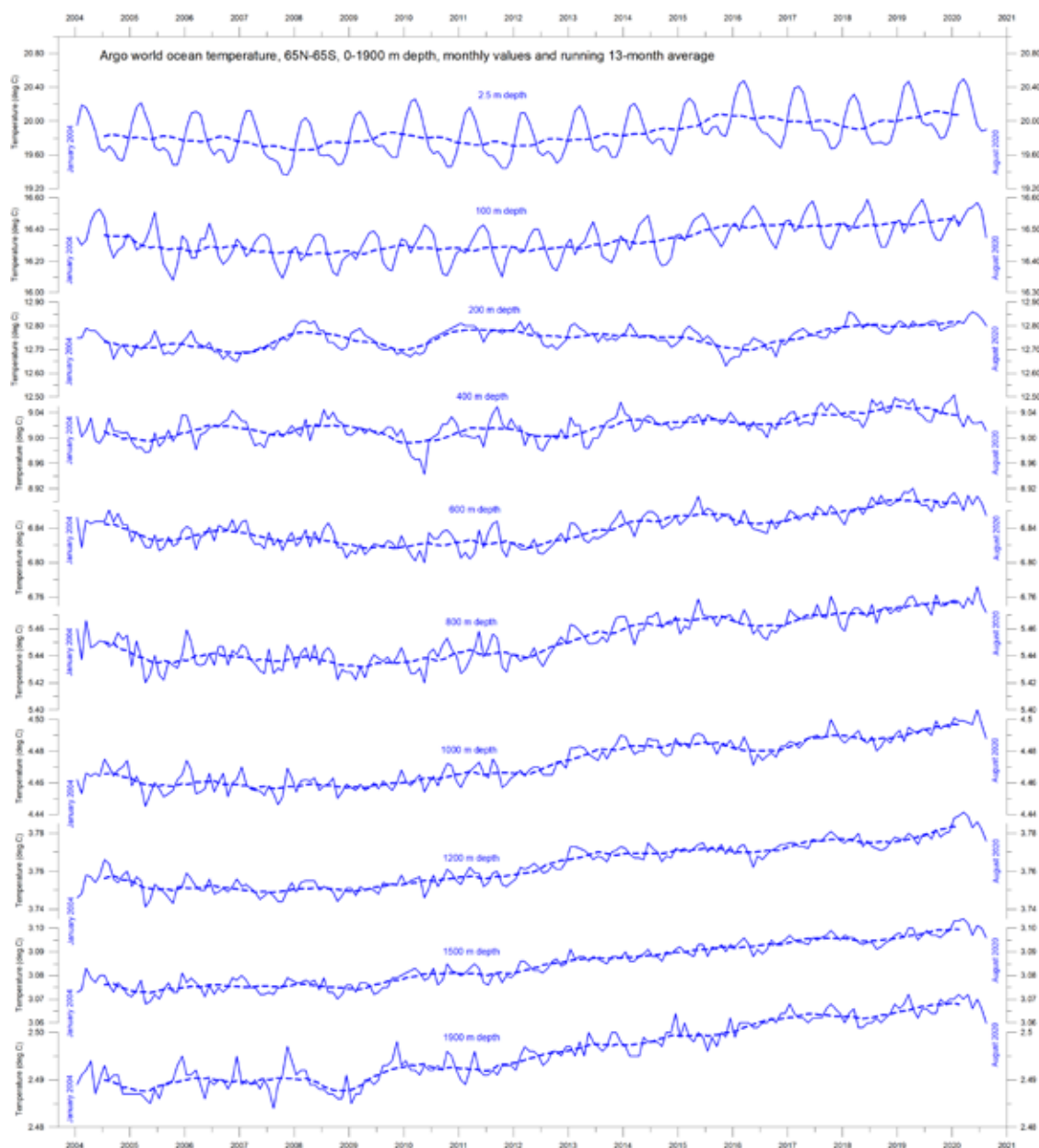
Figure 25: Ocean temperatures at different depths
