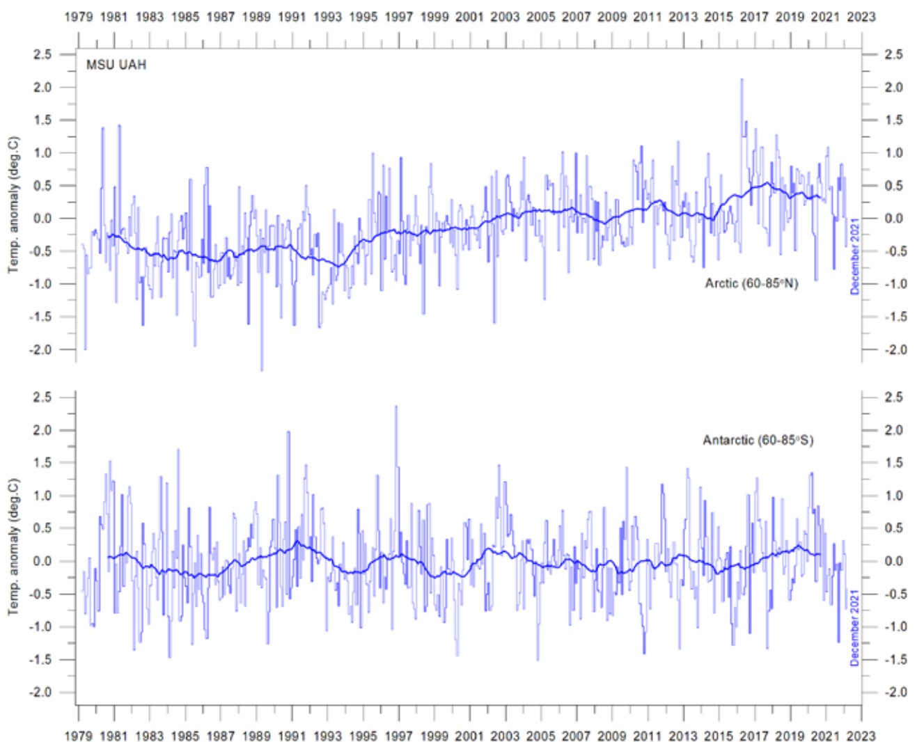
Figure 16: Polar temperatures
