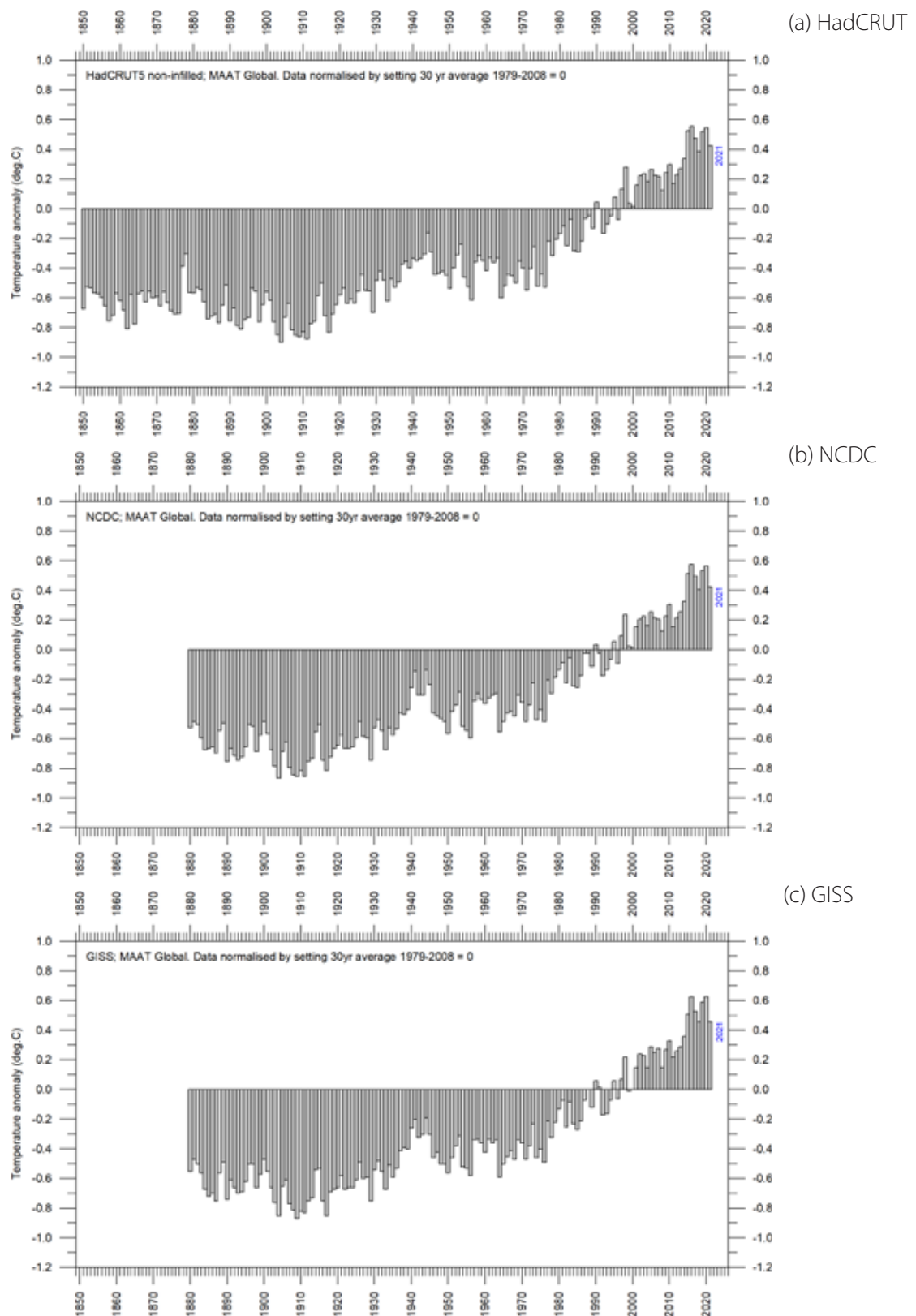
Figure 8: Global mean annual surface air temperatures.
