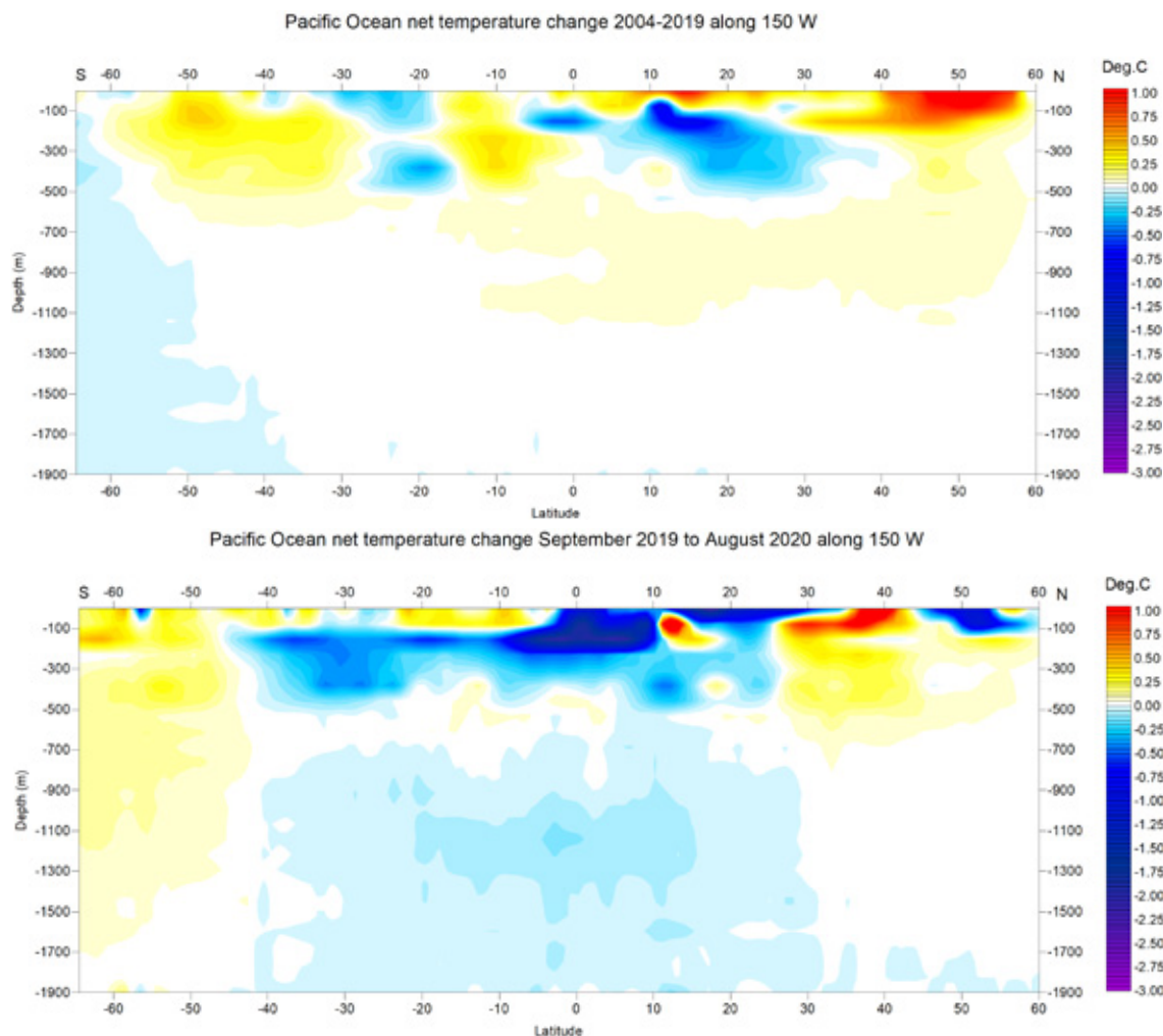
Figure 32: Temperature change along Pacific profile, 0–1900 m
