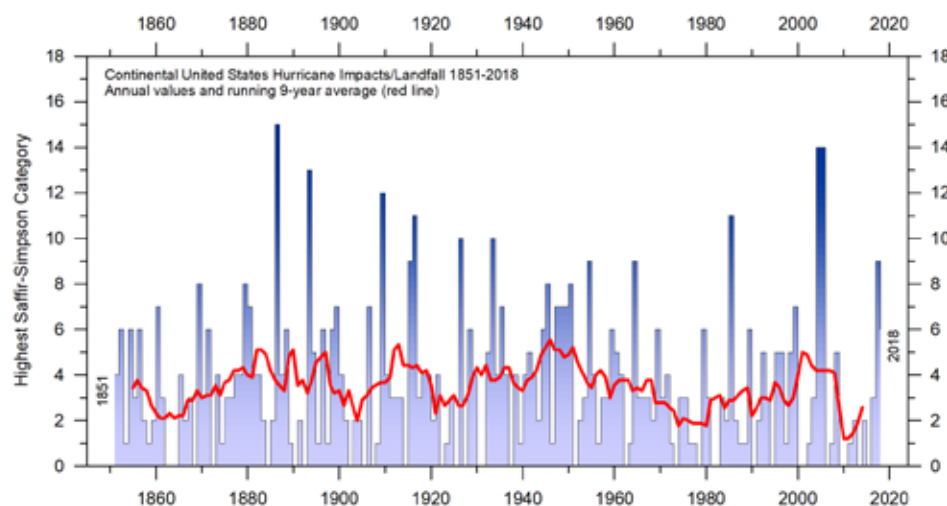
Figure 47: Hurricane landfalls in the continental United States 1851–2018
