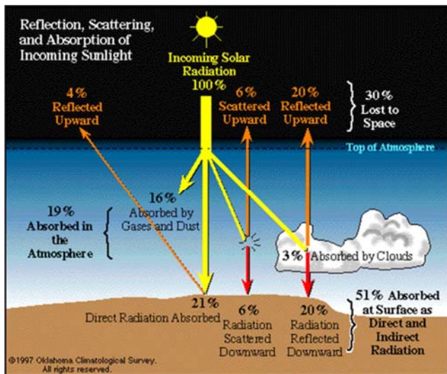
Figure 1. Radiation "Budget" for Incoming Solar Radiation (Oklahoma Climatological Survey) [1].
